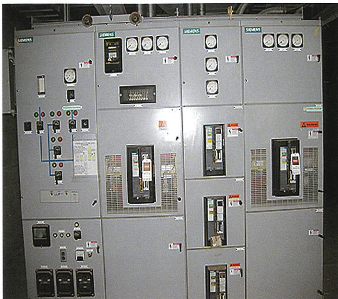
(2) RL3200 (3) RL1600 AIR CIRCUIT BREAKERS
